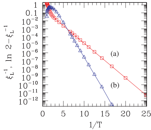
Figure 3. Curve (a): \xi_L^{-1} against 1/T , L = 14 , TM in the F direction. Squares are calculated points; the connecting curve approaches the behaviour \sim \exp(-1/T) from 1/T \simeq 3 onwards. Curve (b): \ln 2 - \xi_L^{-1} against 1/T , L = 14 , TM in the AF direction. Triangles are calculated points; the connecting curve approaches the behaviour \sim \exp(-2/T) from 1/T \simeq 3 onwards.
