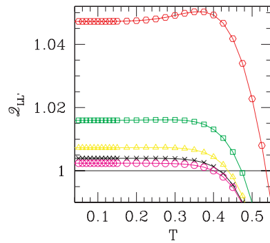
Figure 2. Q_{LL'}(T) of equation (3) against T , for L' = L + 2 . Top to bottom: L = 4, 6, \dots, 12 .
