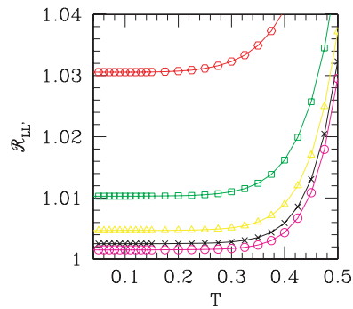
Figure 5. \mathcal{R}_{LL'}(T) of equation (8) against T , for L' = L + 2 . Top to bottom: L = 4, 6, \dots, 12 .
