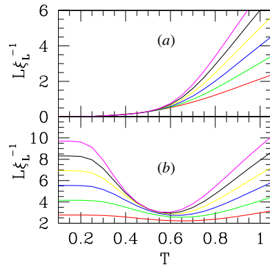
Figure 1. L\xi_L^{-1} against temperature: (a) TM in the ferromagnetic direction; (b) TM in the antiferromagnetic direction. Bottom to top: L = 4, 6, \dots, 14 .
