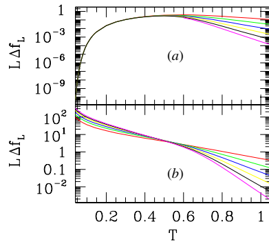
Figure 4. L\Delta f_L against temperature. (a): TM in the ferromagnetic direction. On this scale, curves are indistinguishable up to T \simeq 0.4 ; top to bottom (on the right-hand side): L = 4, 6, \dots, 14 . (b) TM in the antiferromagnetic direction. Curves cross in the central region of the T axis. Top to bottom (on the right-hand side): L = 4, 6, \dots, 14 .
