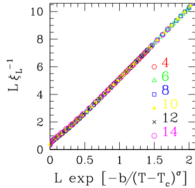
Figure 6. Scaling plot (see equation (10)) of the data displayed in figure 1(a). The parameters are: T_c = 0.51 , b_\xi = 1.60 , \sigma = 0.54 (see the text).
